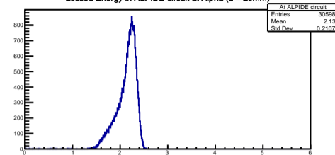
Lossed Energy in ALPIDE circuit at Alpha (d = 29mm)
